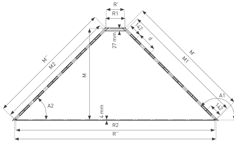
R' min = 200 mm, R'' max = 6300 mm, A1 = 90.1° to 135°, A2 = 45° to 89.9°
