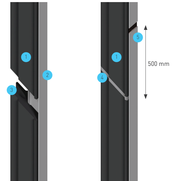
Extending the rubber sealing profile
