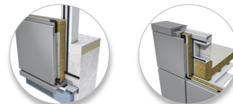
BASE DETAIL TOP PARAPET DETAIL
