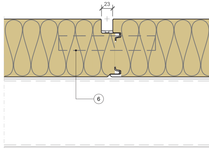
VERTICAL CUT
