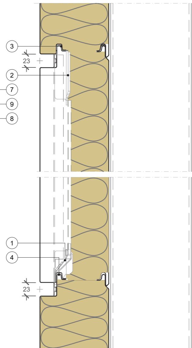
VERTICAL CUT
