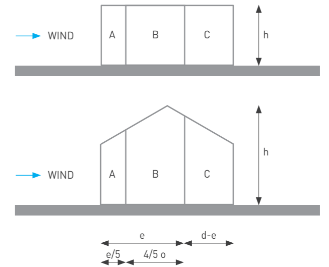
Side-plan for e < d .
