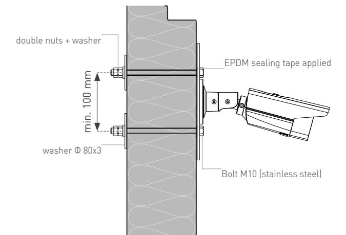
Fixing through the element with M10 bolt (stainless steel), a large washer and double nuts.
