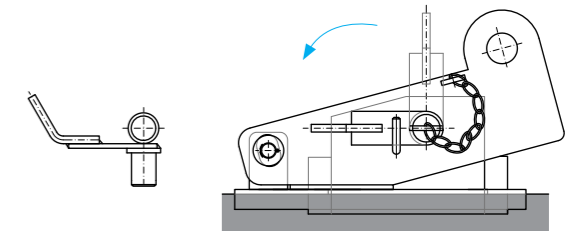
Insertion of a safety pin.
