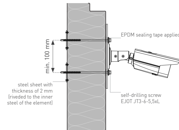
Fixing through the element to a 2 mm steel sheet attached to the internal steel sheet.
