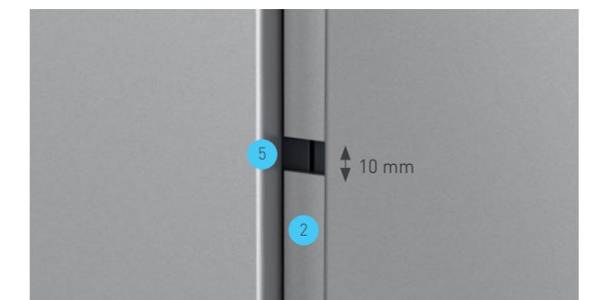
Extending the decorative Alu. extrusion HF40
