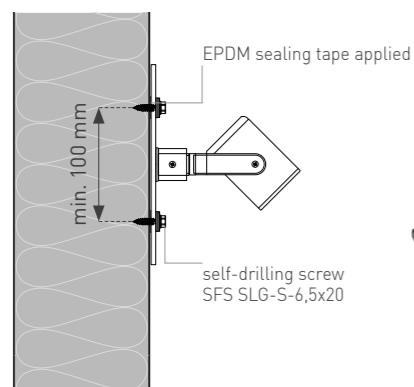
Fixing with self-drilling screws
