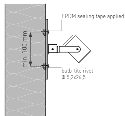
Fixing with rivets
