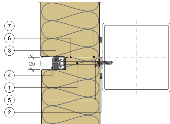
VERTICAL CUT
