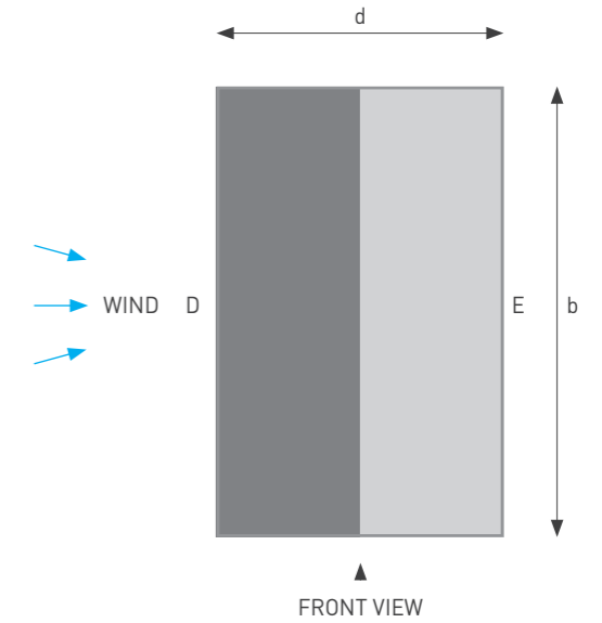
Determining edge zones on a simple rectangular building with proportions e < d .
